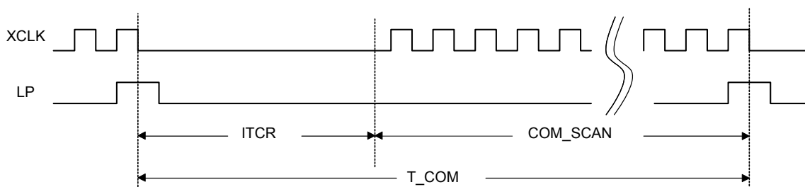
Figure 6-29 : Scan for Each COM Line
