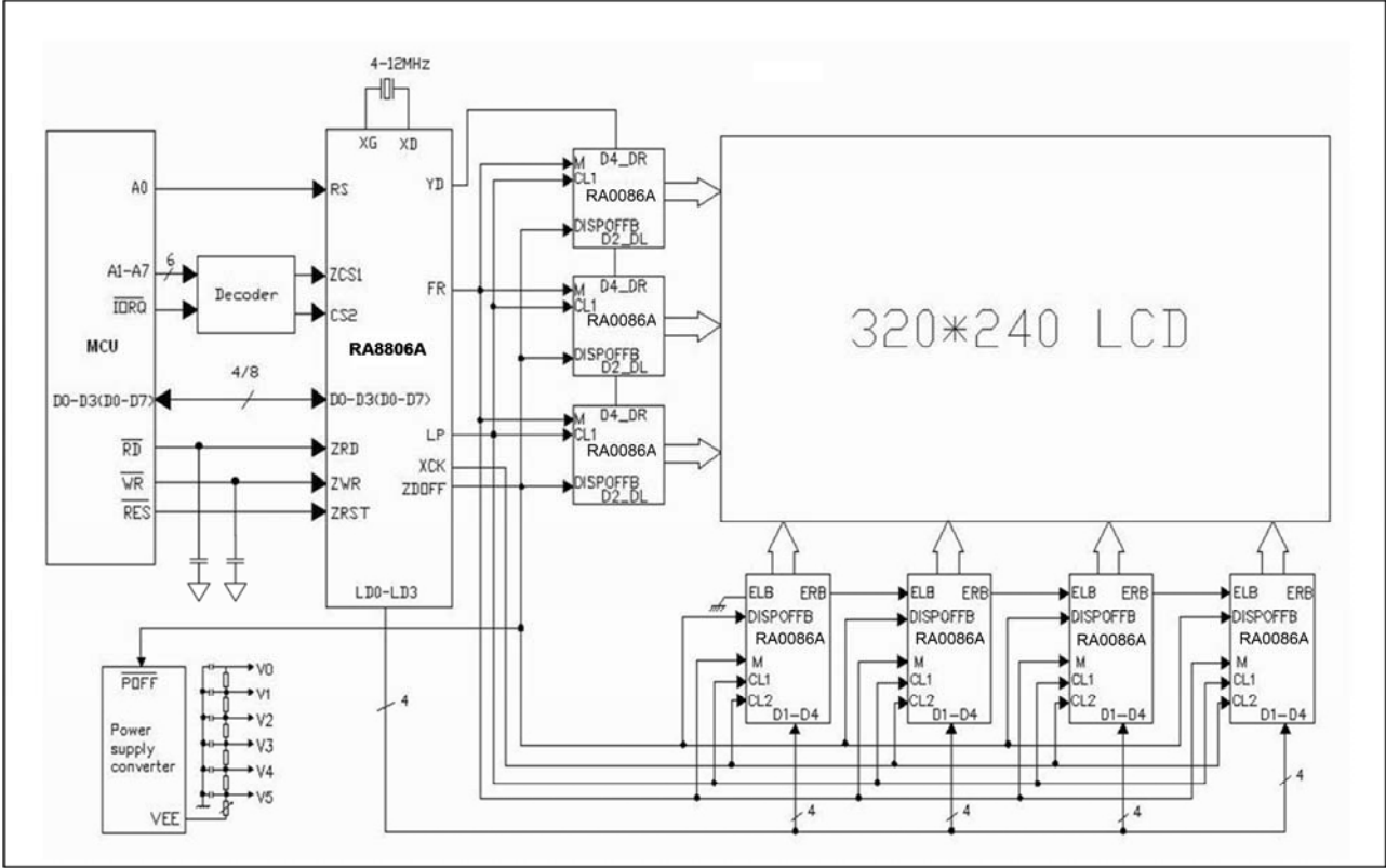
Figure 6-10 : Application Circuit Diagram for 320x240 Panel
