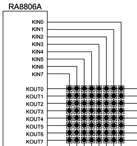
Figure 6-16 : 8x8 Key-Pad Application
