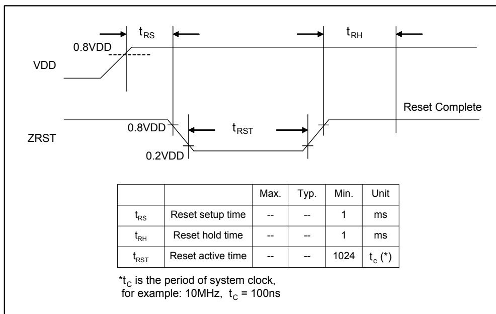
Figure 6-22 : Reset Timing
