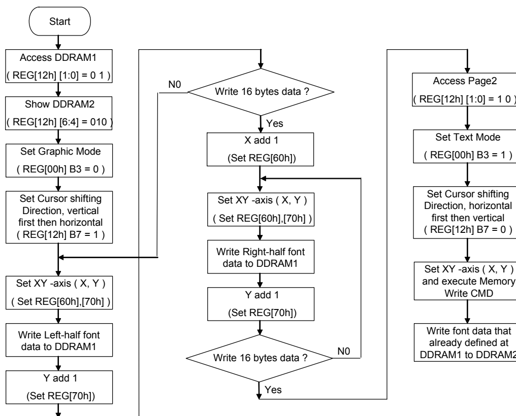
Figure 6-48 : Flowchart of User-created font in DDRAM1
