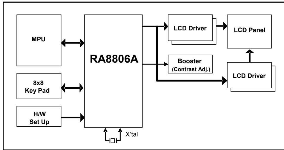
Figure 3-2 : RA8806A System Block Diagram
