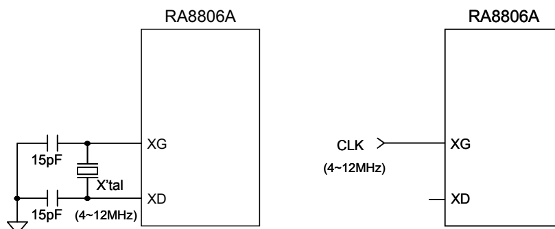
Figure 6-19 : Clock Circuit
