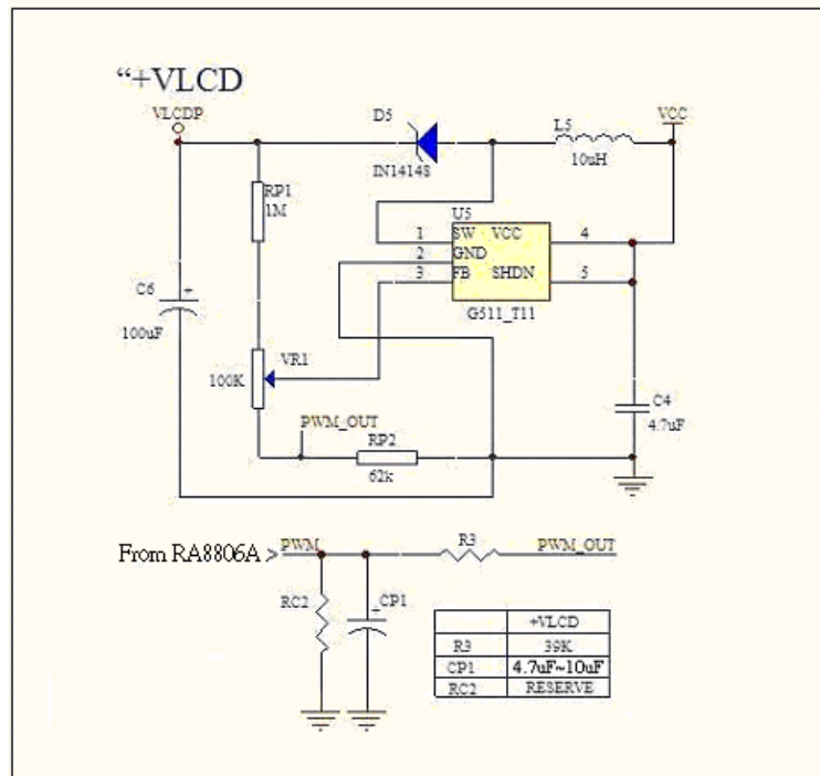
Figure 6-32 : PWM Reference Circuit for Positive VLCD
