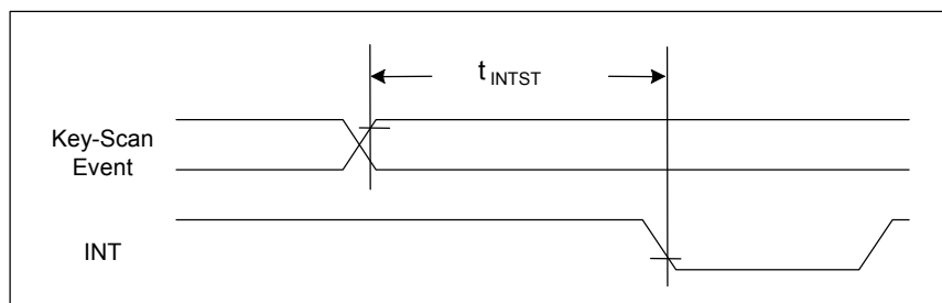
Figure 6-27 : Interrupt Timing(2)
