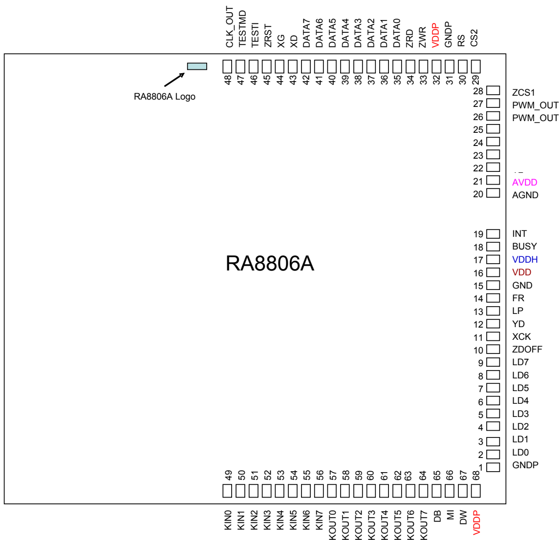
Figure 7-1 : RA8806A Bonding Pad
