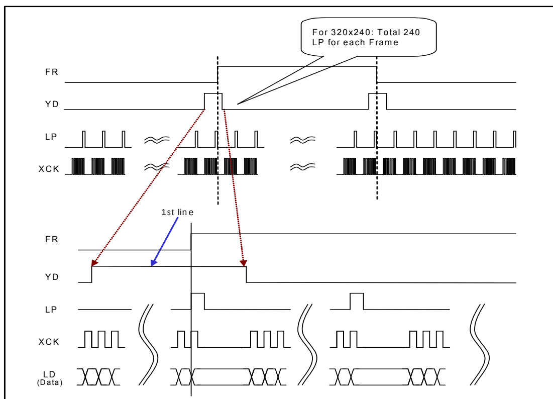
Figure 6-9 : The Waveform of RA8806A and LCD Driver
