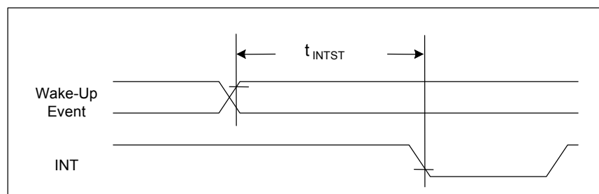
Figure 6-26: Interrupt Timing(1)
