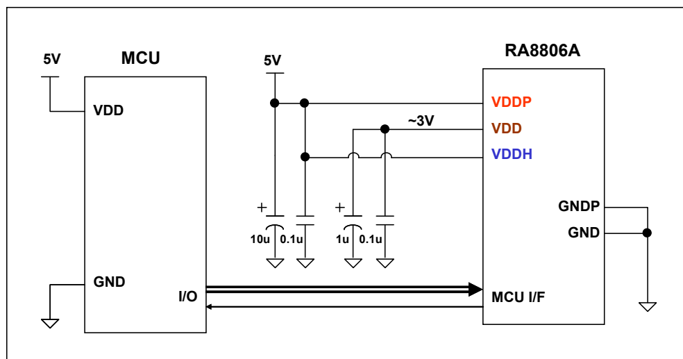
Figure 6-25 : The Power Connection of 5V
