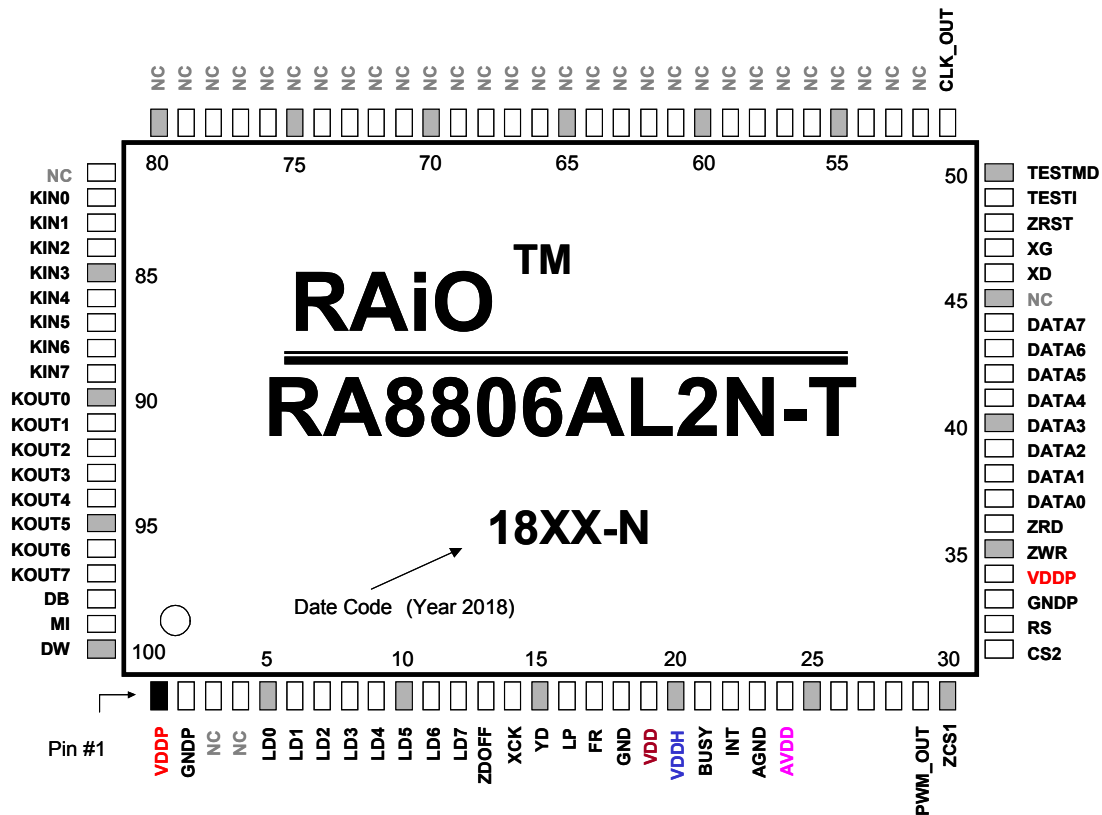
Figure 7-2 : LQFP-100Pin Pin Assignment
