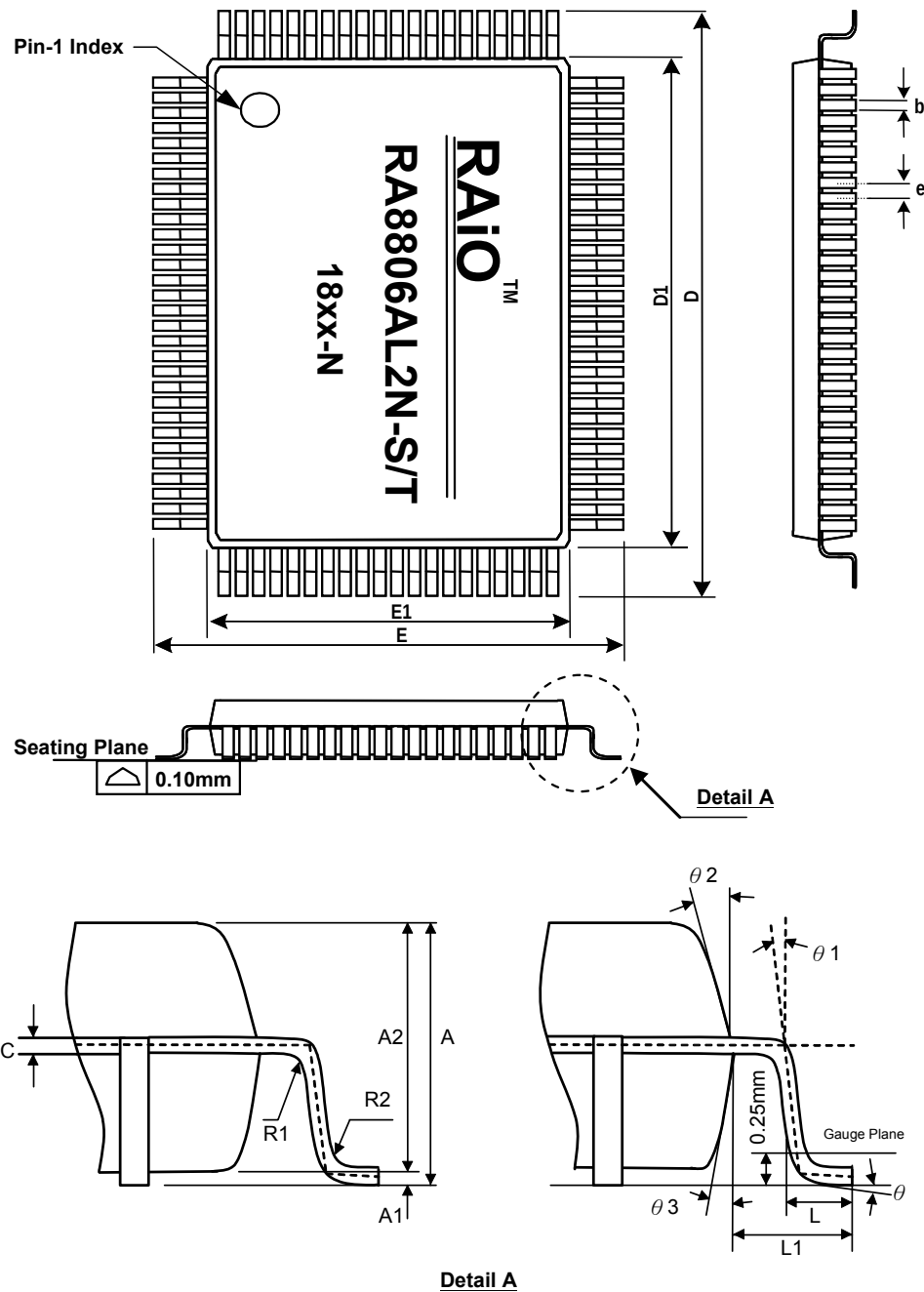
Figure 7-3 : LQFP-100Pin Mechanical
