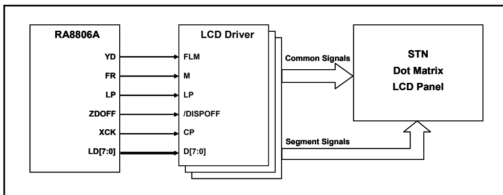
Figure 6-8 : The Interface of RA8806A and LCD Driver
