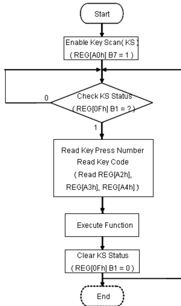
Figure 6-17 : Key-Scan Flowchart (1)
