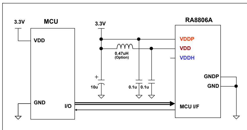
Figure 6-24: The Power Connection of 3V
