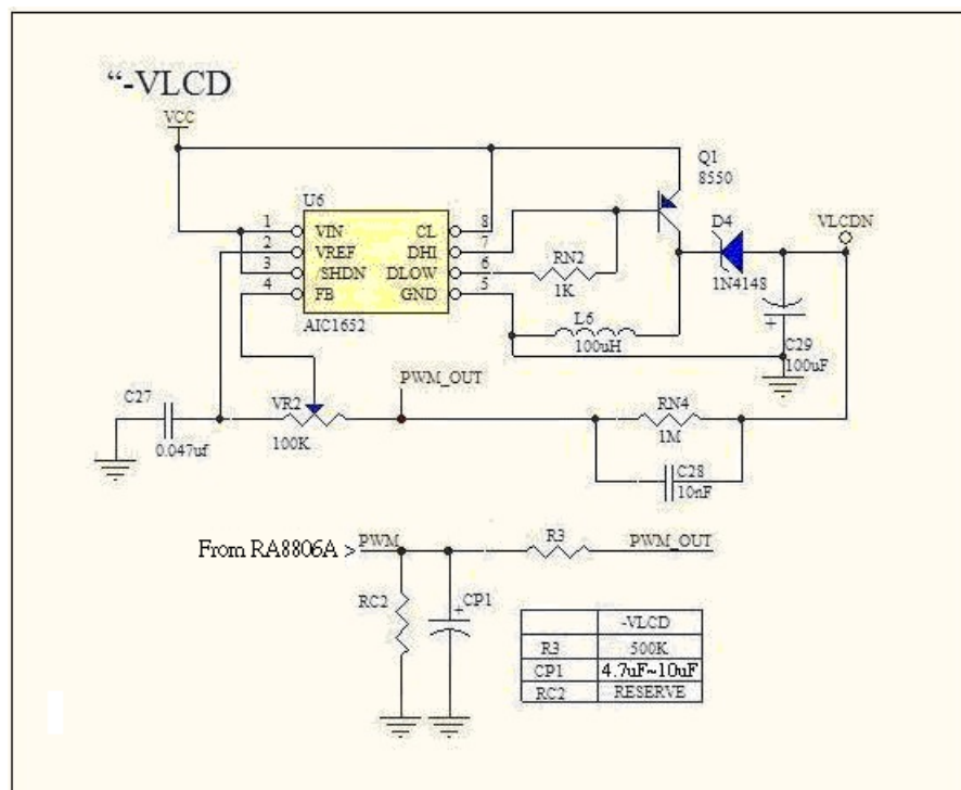
Figure 6-33 : PWM Reference Circuit for Negative VLCD
