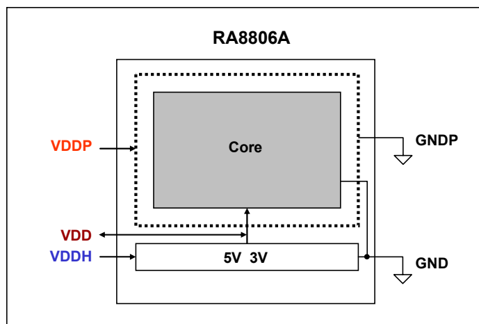
Figure 6-23 : Power Architecture
