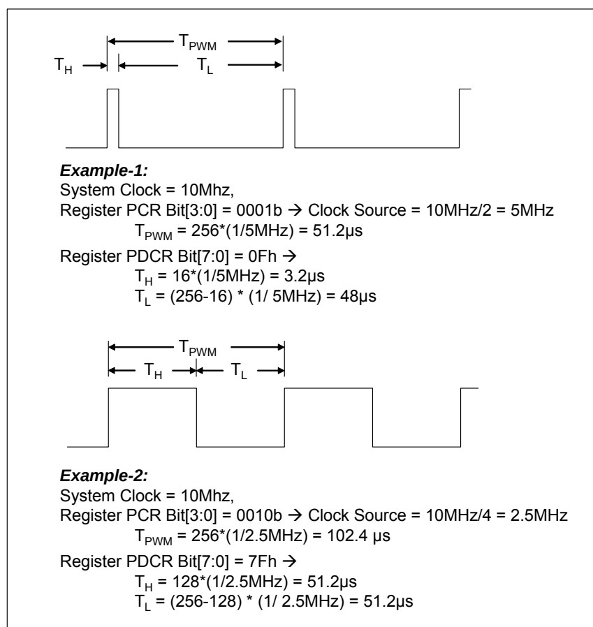
Figure 6-31 : PWM_OUT Pulse
