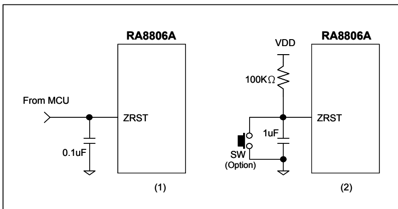
Figure 6-21: Examples of ZRST Pin
