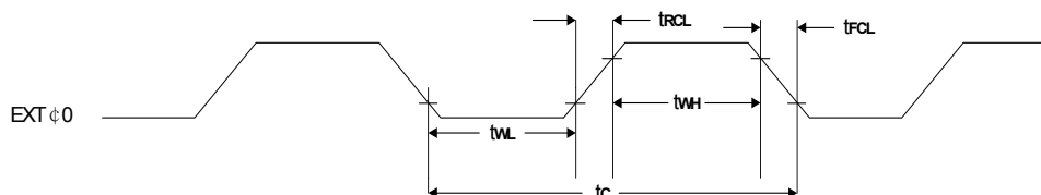
Figure 6-20 : External Clock
