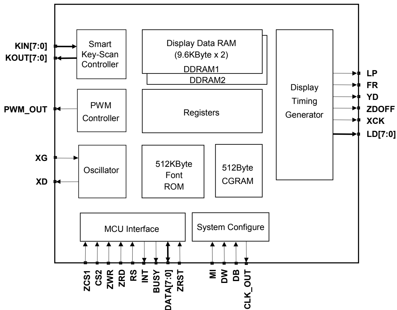
Figure 3-1 : RA8806A Block Diagram
