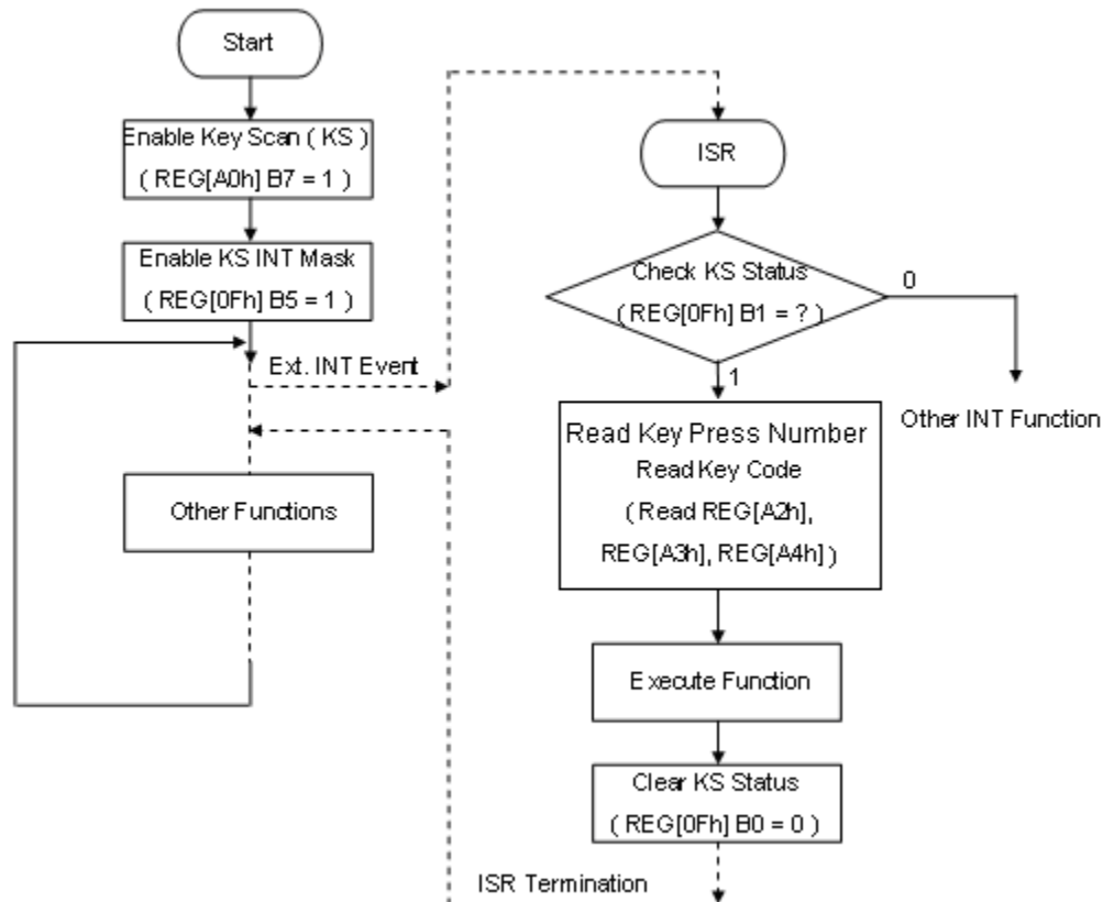
Figure 6-18 : Key-Scan Flowchart (2)
