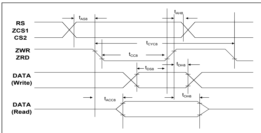
Figure 6-3 : 8080 MPU Interface Waveform
