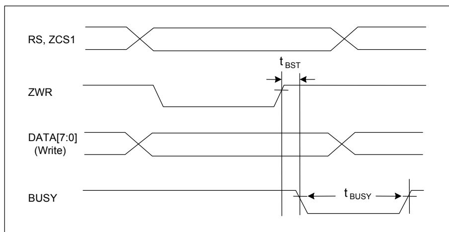
Figure 6-30 : BUSY Timing Chart
