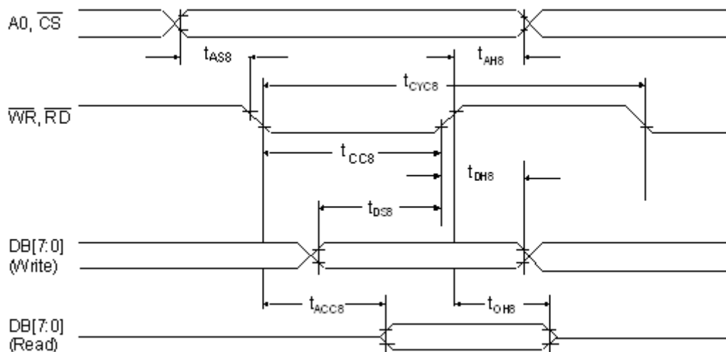
Figure 6-4 : 8080 Waveform
