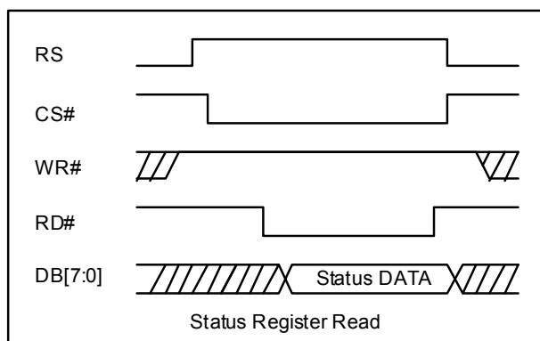
Figure 6-26 : 8080 Read Status Register
