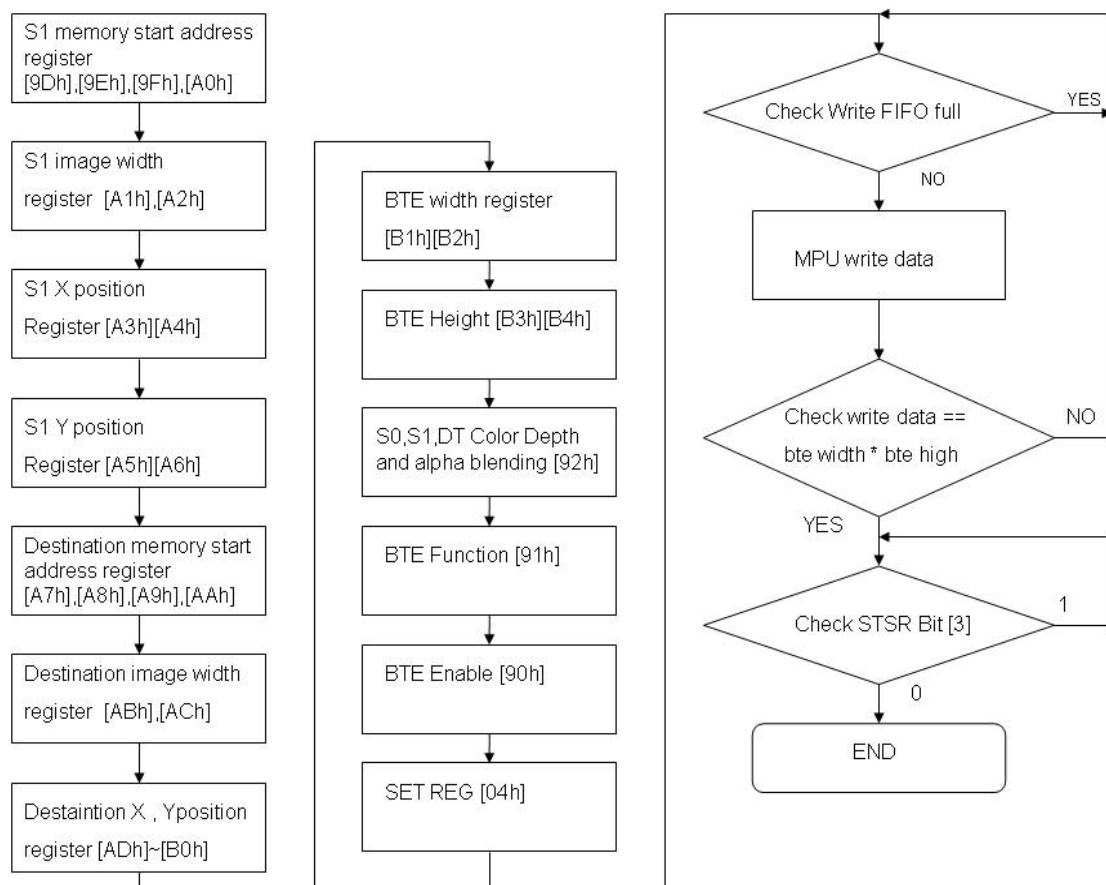
Figure 13-32 : Flow Chart
