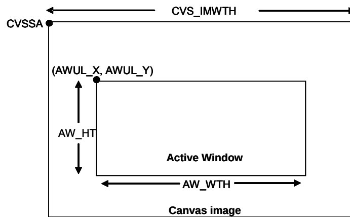
Figure 19-4 : Active Window
