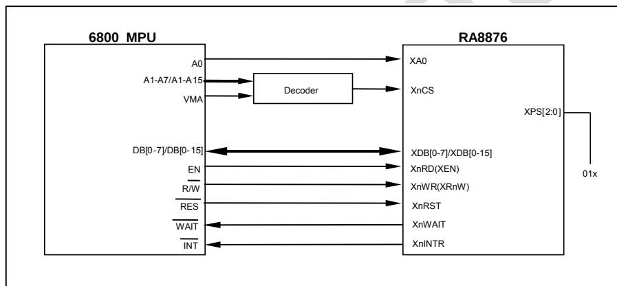
Figure 7-2 : 6800 MCU Interface
