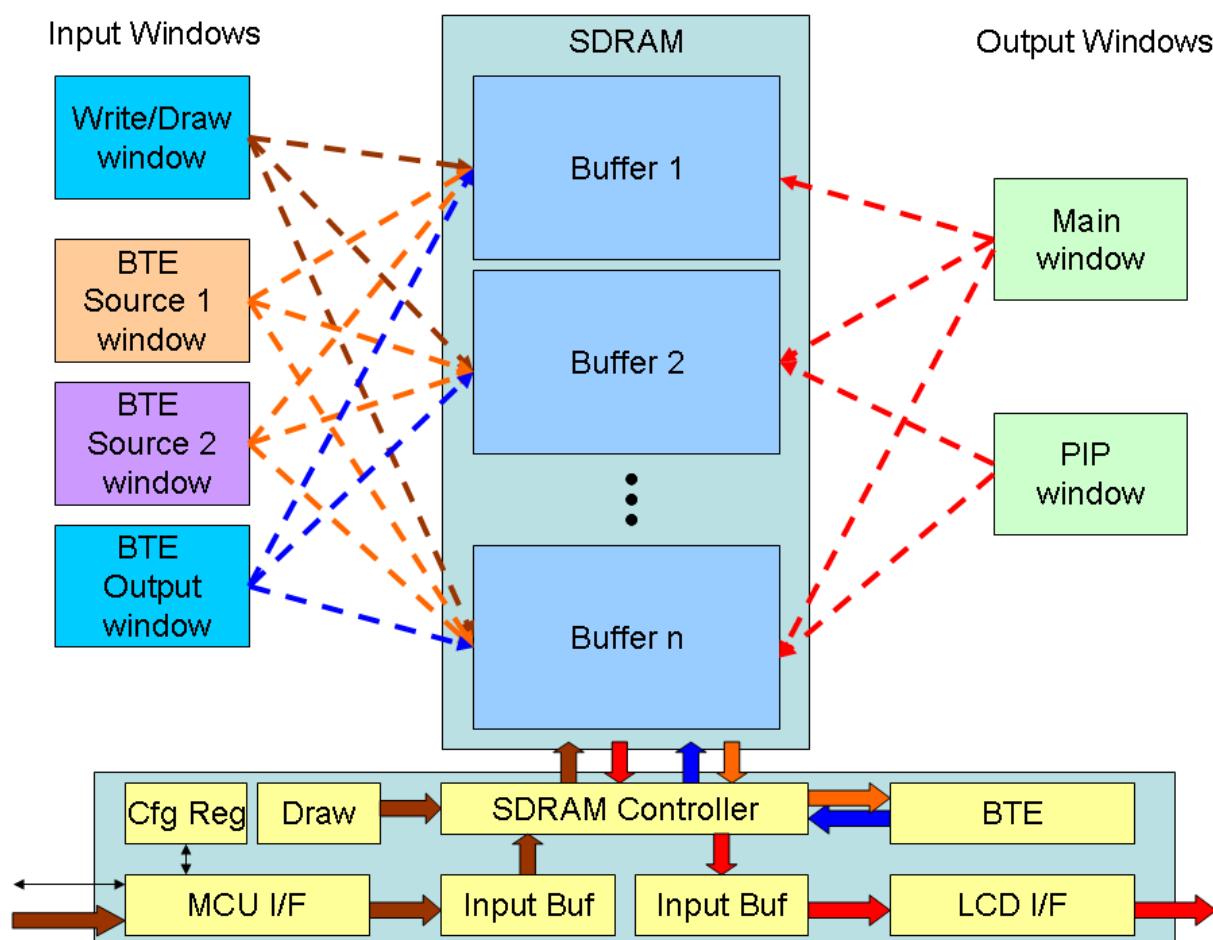
Fig.9- 1 Display Data path
