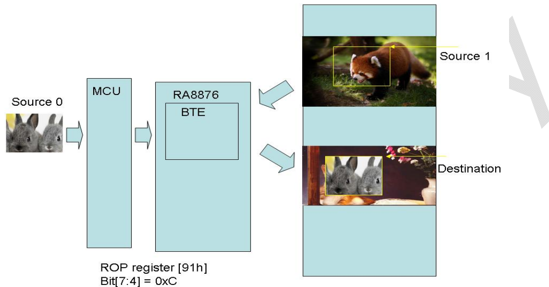
Figure 13-5 : Hardware Data Flow
