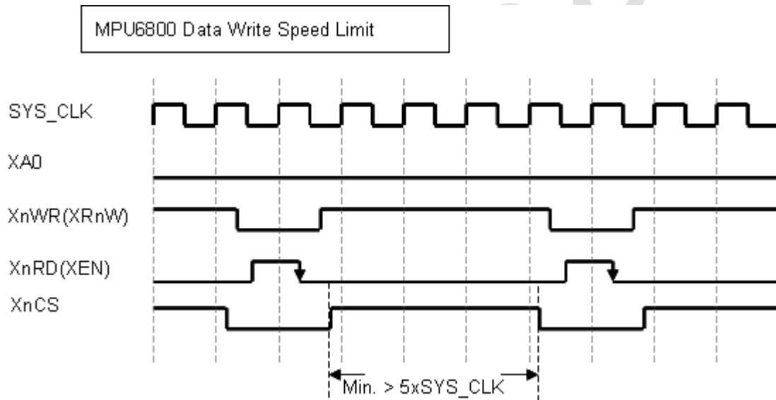
Figure 7-6 : 6800 I/F Continuous Data Write Cycle Waveform
