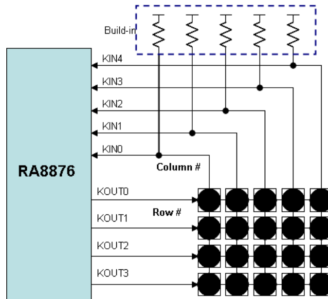
Figure 17-1 : Key-Pad Application
