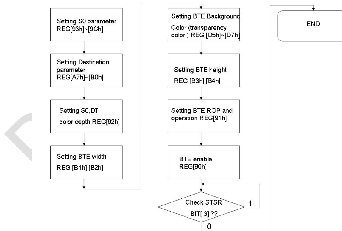
Figure 13-17 : Hardware Flow
