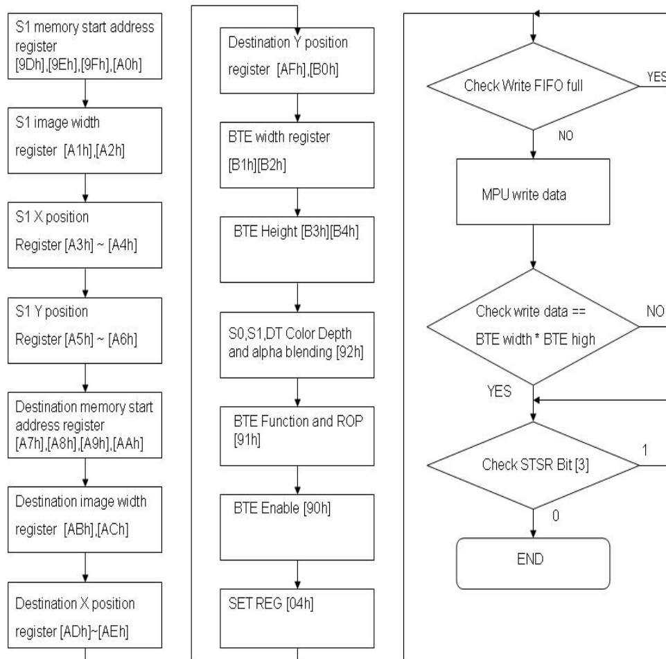
Figure 13-6 : Flow Chart
