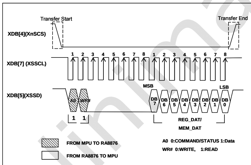
Figure 7-10 : Data Read on 3-Wire SPI-Bus
