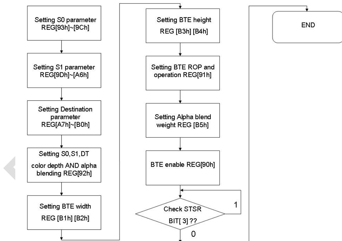
Figure 13-30 : Picture Mode Flow Chart
