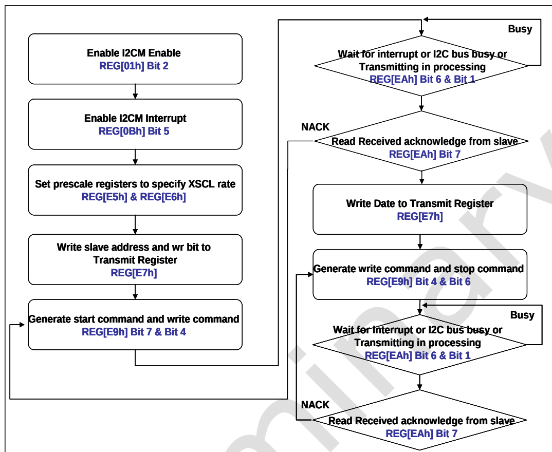
Figure 16-16 : Flow for Write 1 Byte Data to Slave
