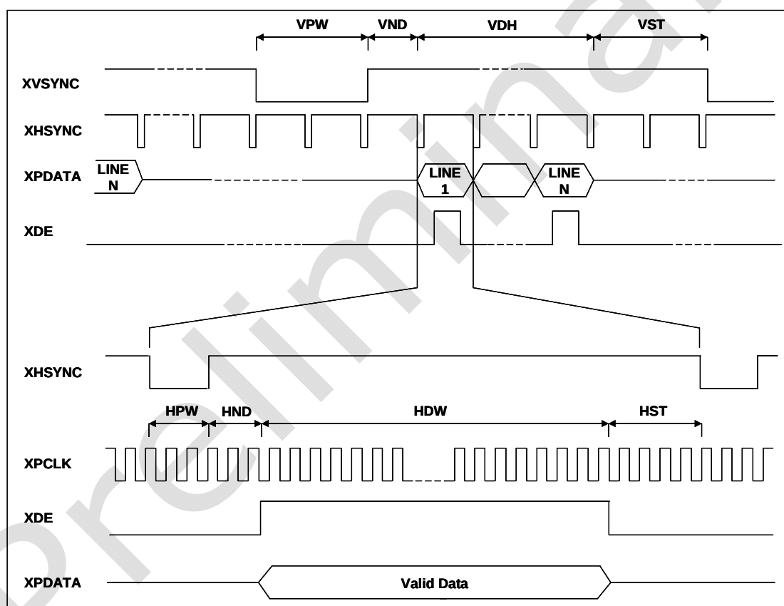
Figure 19-3 : Digital TFT Panel Timing
