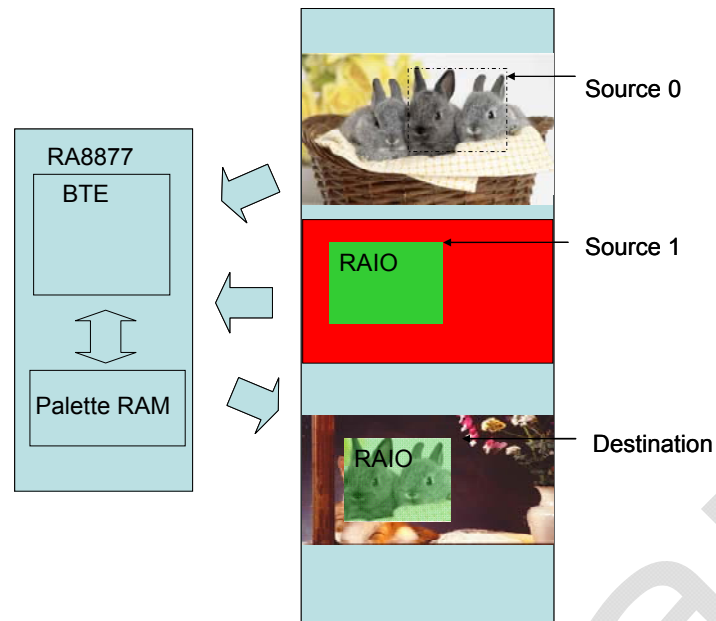
Figure 13-26 : 8bpp Pixel mode Hardware Data Flow
