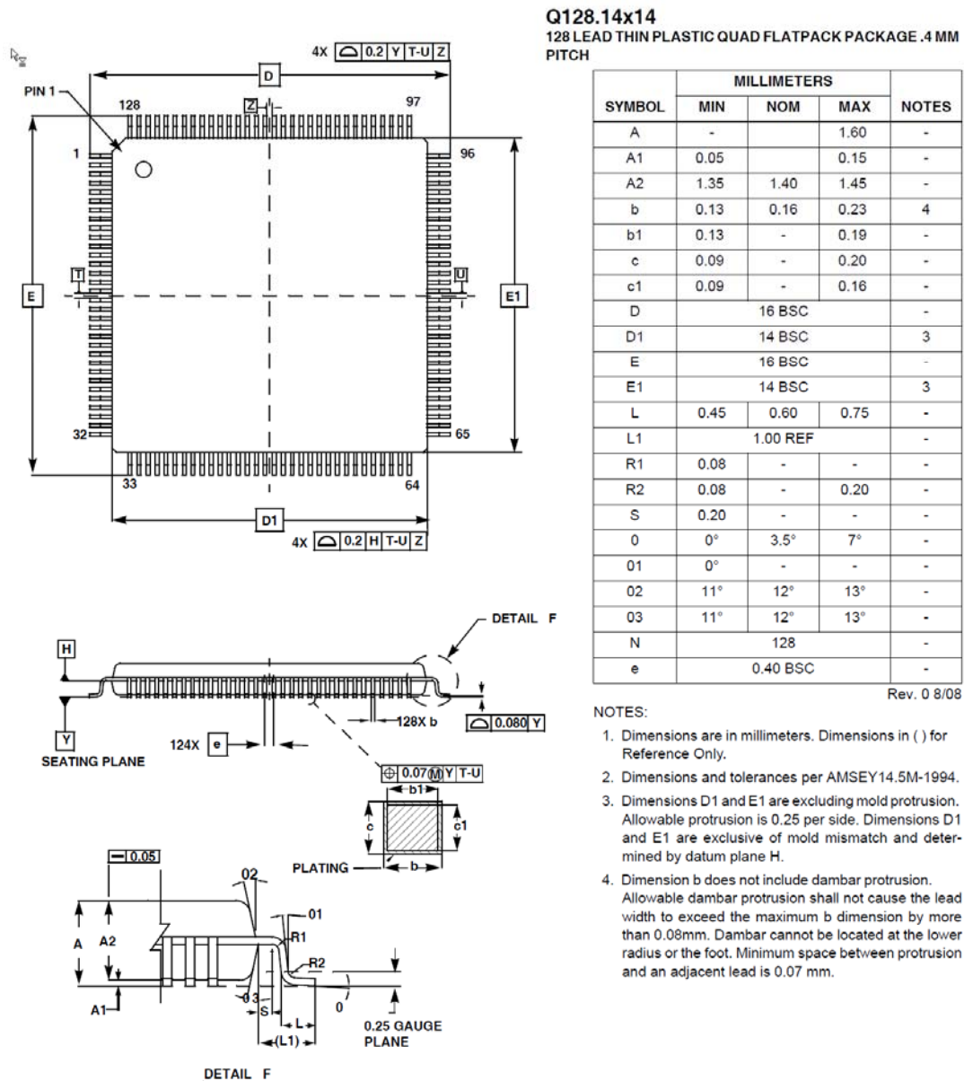
Figure 3-2 : RA8877 Package Outline Dimensions
