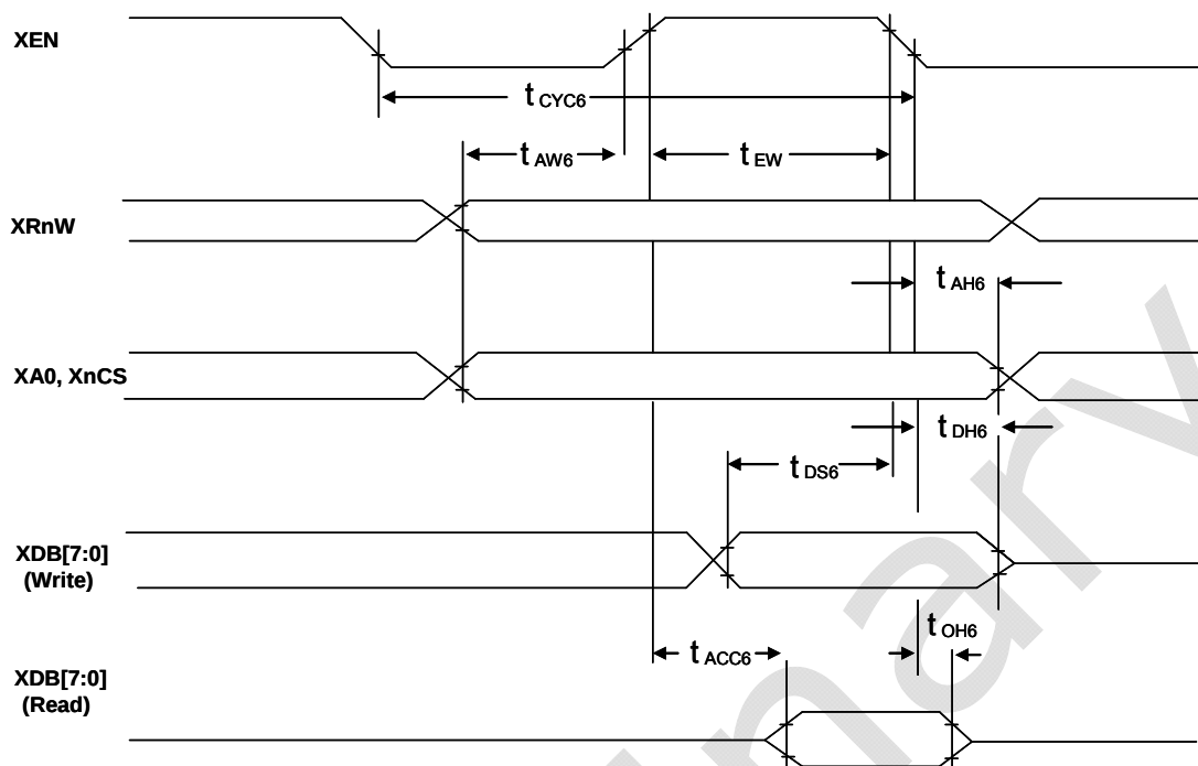
Figure 7-4 : 6800 MCU Waveform
