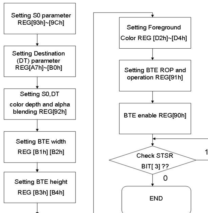
Figure 13-38 : Flow Chart
