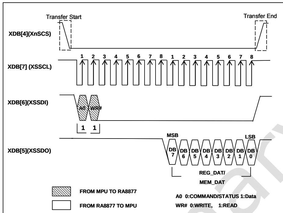
Figure 7-14 : Data Read on 4-Wire SPI-Bus
