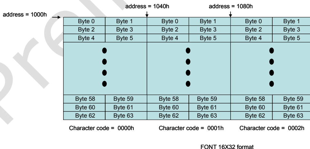
Figure 14-8 : Font 16x32 Array in SDRAM
