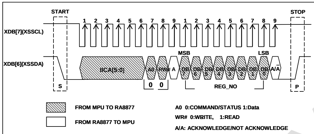
Figure 7-20 : CMD Write on IIC-Bus
