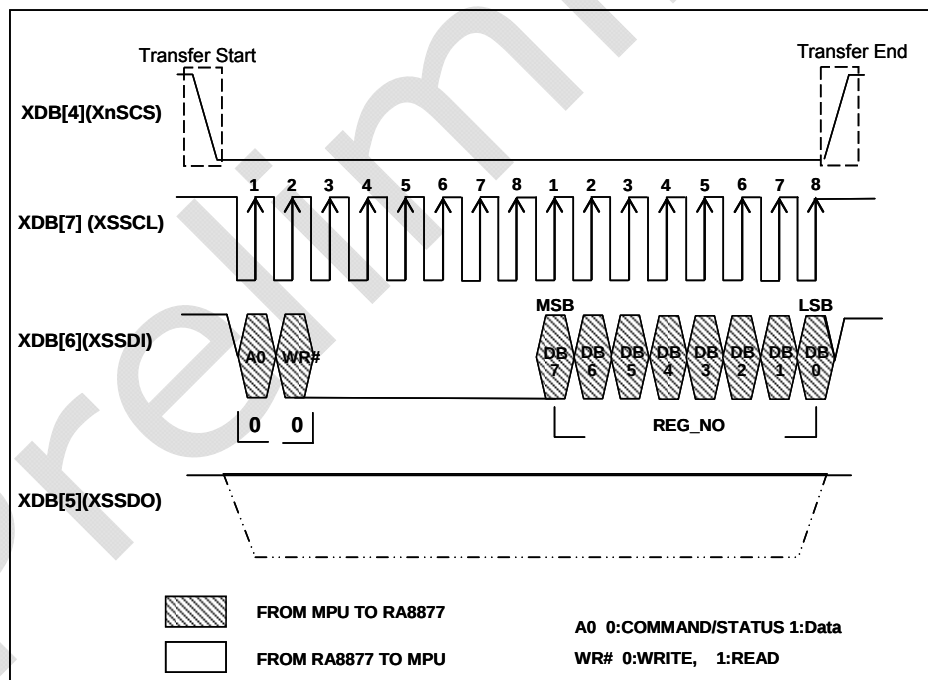
Figure 7-15 : CMD Write on 4-Wire SPI-Bus
