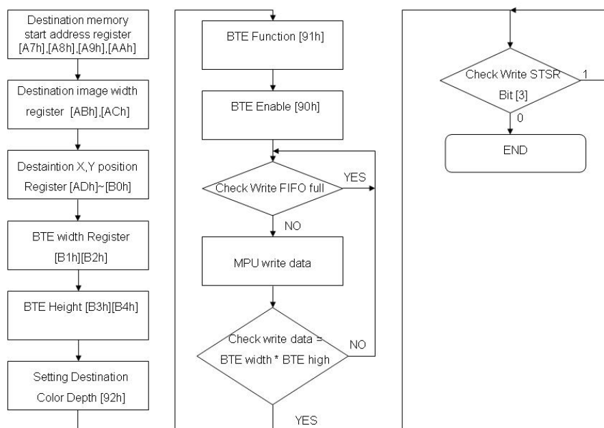
Figure 13-19 : Hardware Data Flow
