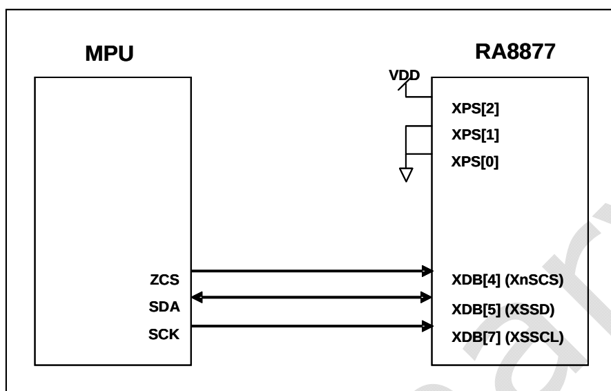
Figure 7-7 : The MCU Interface Diagram of 3-Wire SPI
