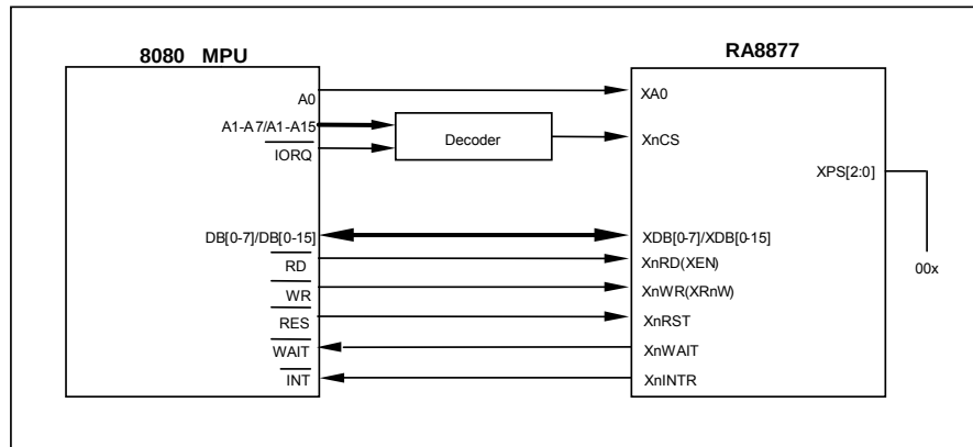
Figure 7-1 : 8080 MCU Interface
