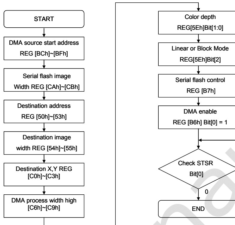
Figure 16-13 : Enable DMA Procedure – Check Flag
