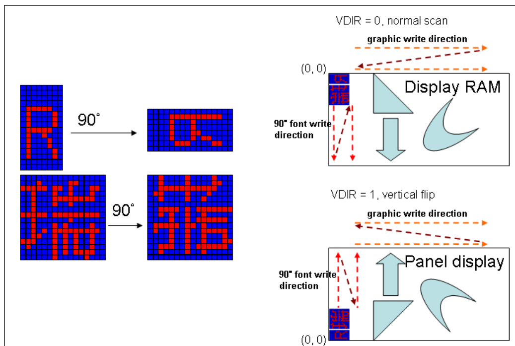
Figure 14-12: Rotation 90° Characters
