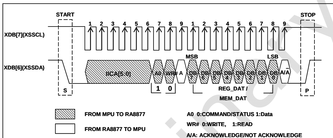
Figure 7-18 : Data Write on IIC-Bus
