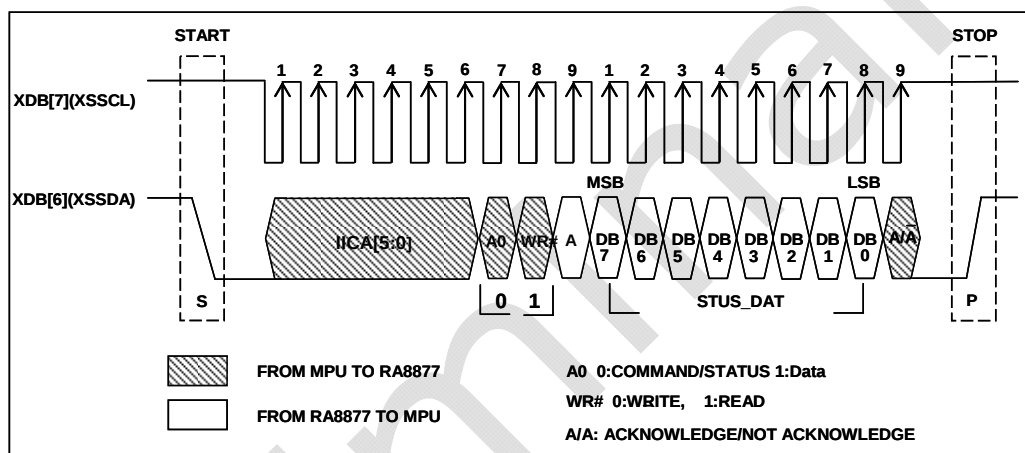
Figure 7-21 Status Read on IIC-Bus
