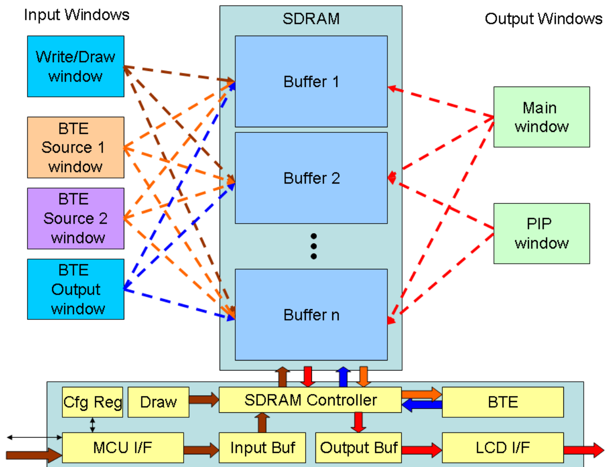
Fig.9- 1 Display Data Path
