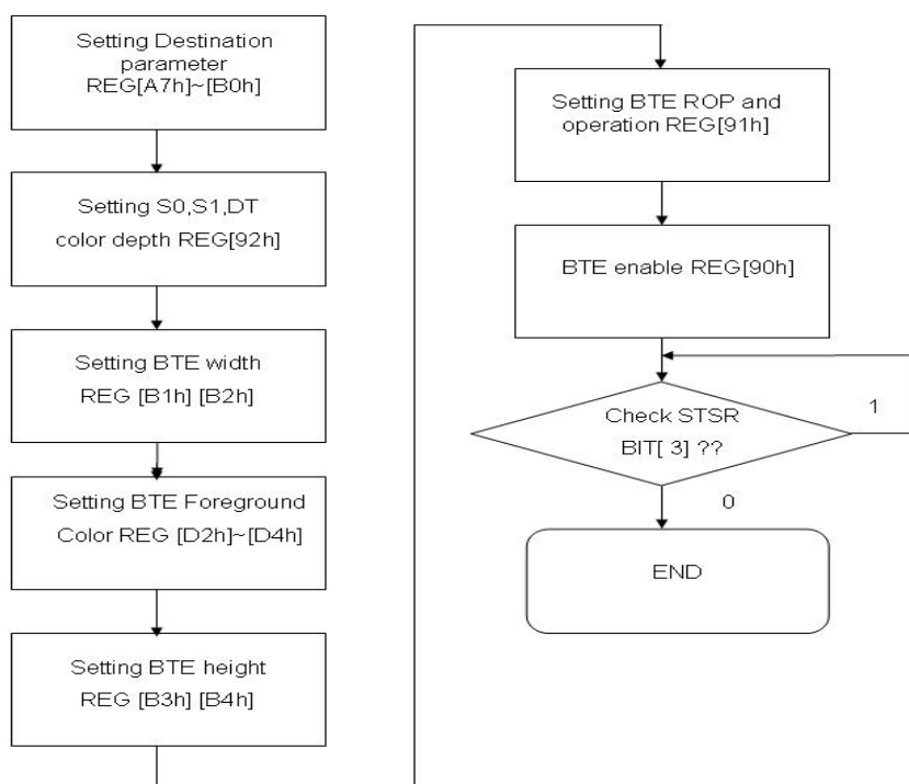
Figure 13-40 : Flow Chart
