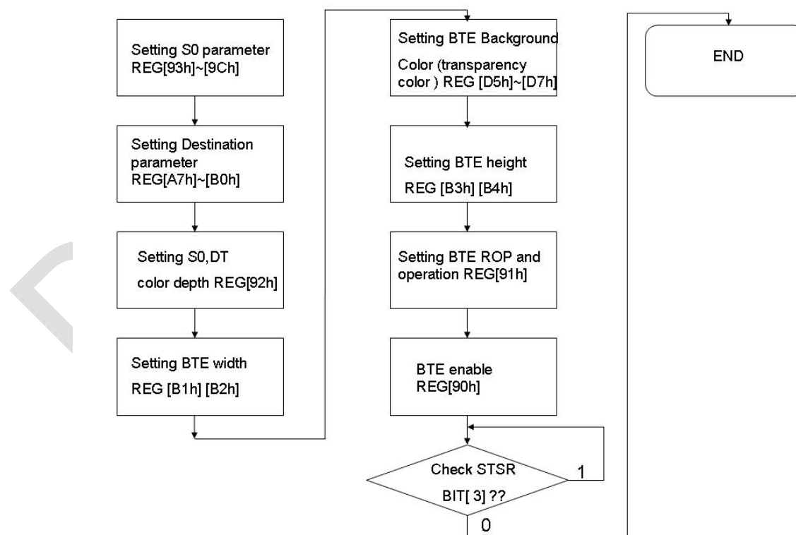
Figure 13-18 : Flow Chart
