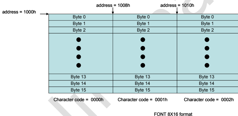
Figure 14-4 : Font 8X16 Array in SDRAM
