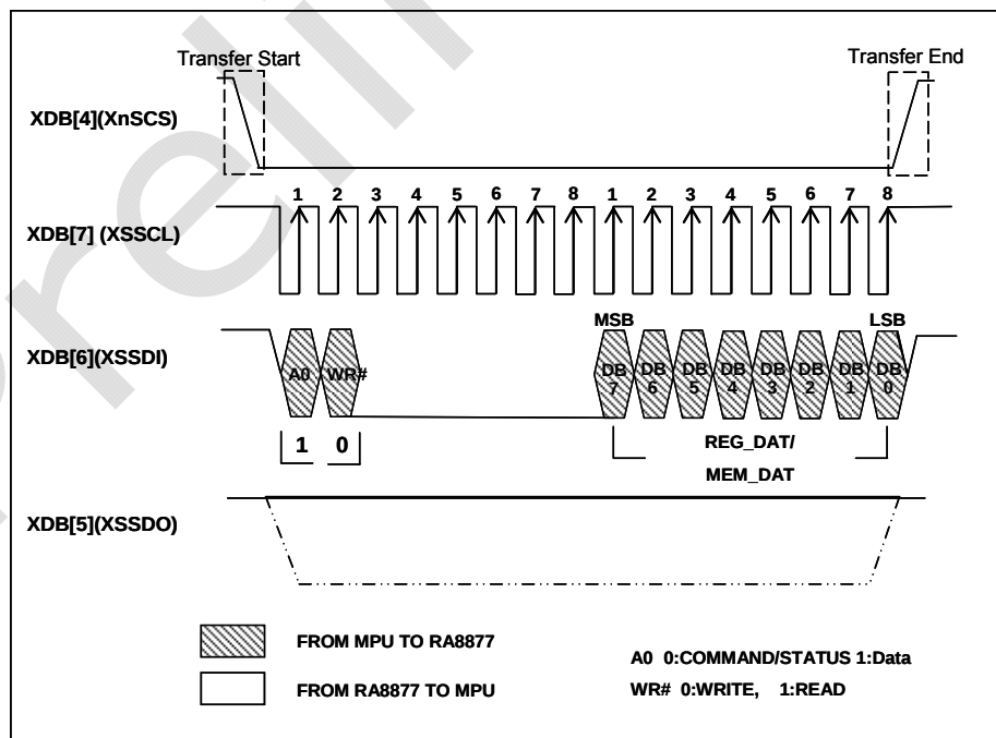
Figure 7-13 : Data Write on 4-Wire SPI-Bus
