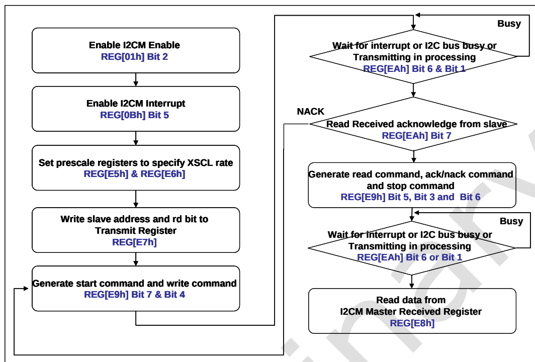
Figure 16-18 : Flow for Read 1 Byte Data from Slave
