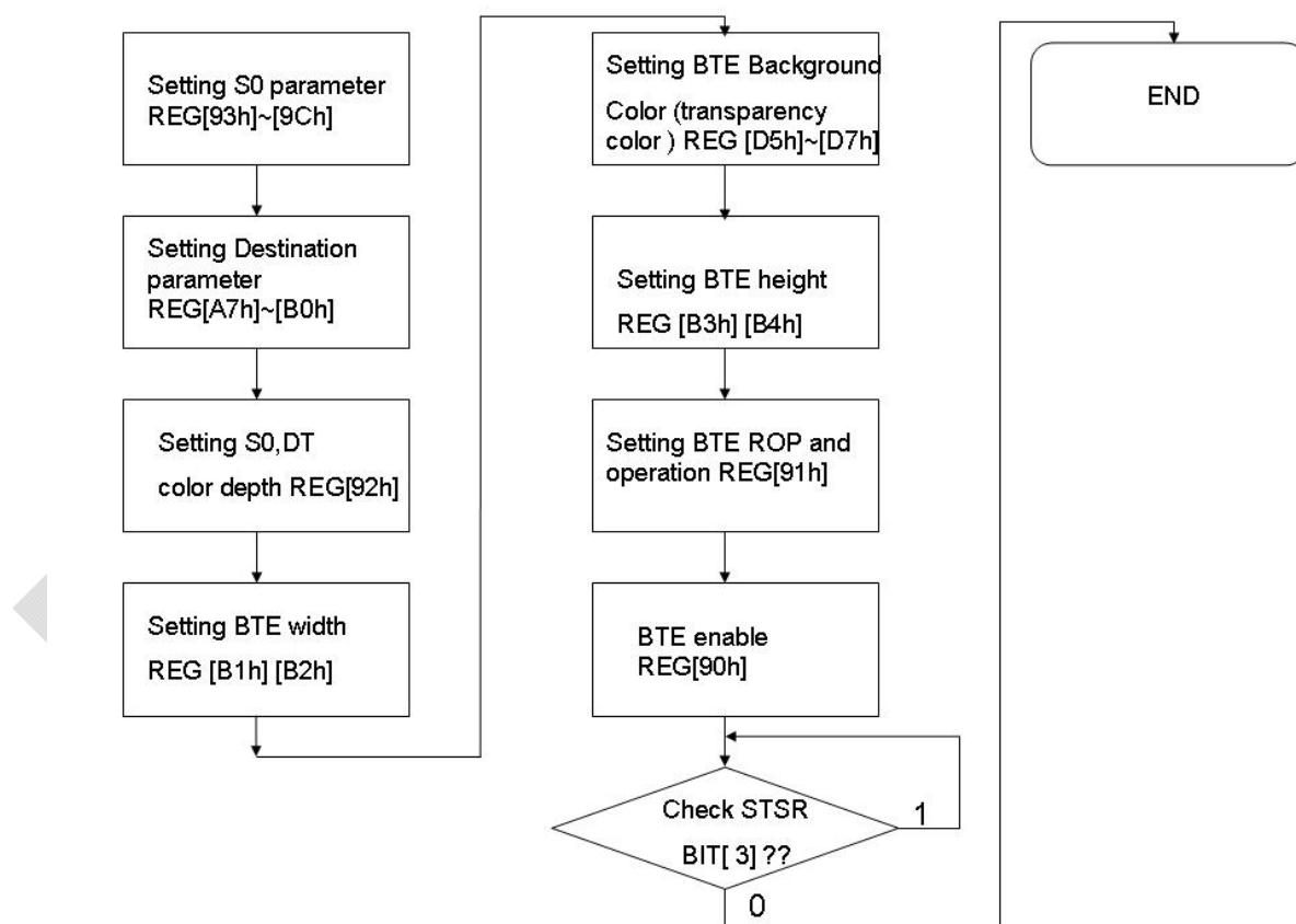
Figure 13-12 : Flow Chart
