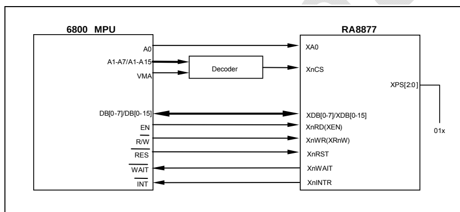
Figure 7-2 : 6800 MCU Interface
