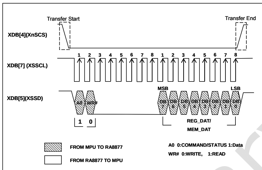
Figure 7-11 : Date Write on 3-Wire SPI-Bus
