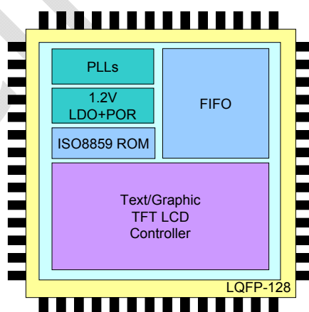
Figure 1-2 : Chip Diagram
