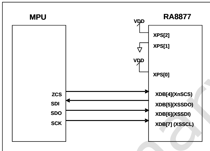
Figure 7-12 : The MCU Interface Diagram of 4-Wire SPI
