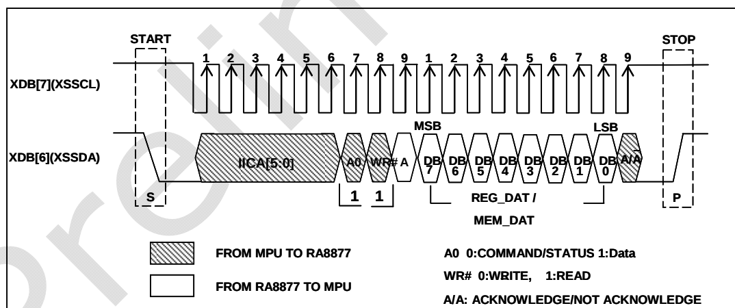
Figure 7-19 : Data Read on IIC-Bus
