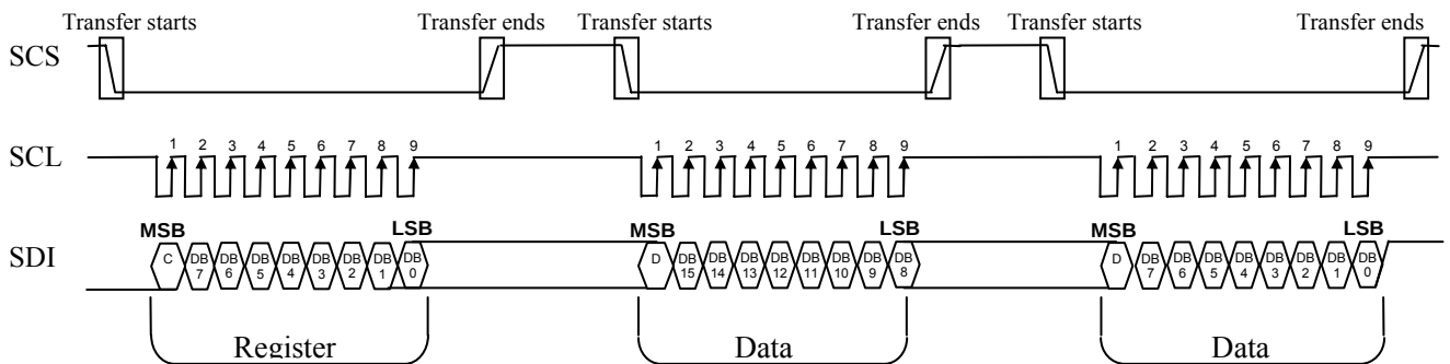
Figure 7-3: 3-wire SPI interface (9 bits)
