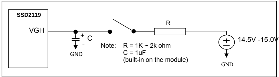
Figure 9-3: OTP circuitry
