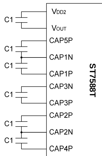
6x step-up voltage circuit
